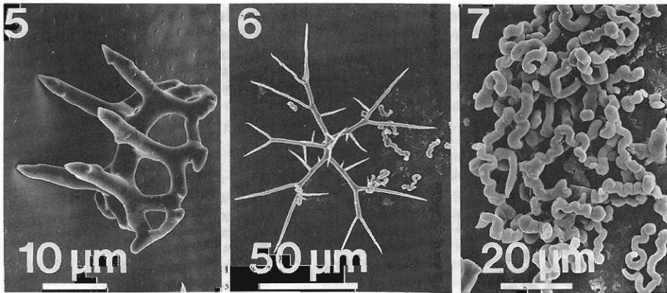
Figures 5 to 7. Spicules of Thelenota rubralineata n. sp. 5. Pseudo-table; 6. Dichotomous rod; 7. Serpent-like miliary granules.
