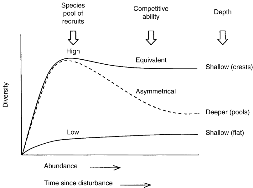
FIG. 11. Hypotheses of the relationship of species diversity to variation in abundance in different environments, either in a series of samples or during recovery of abundance following a drastic disturbance.
